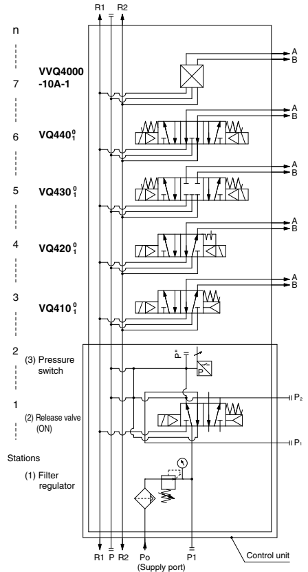
Circuit of control unit manifold
